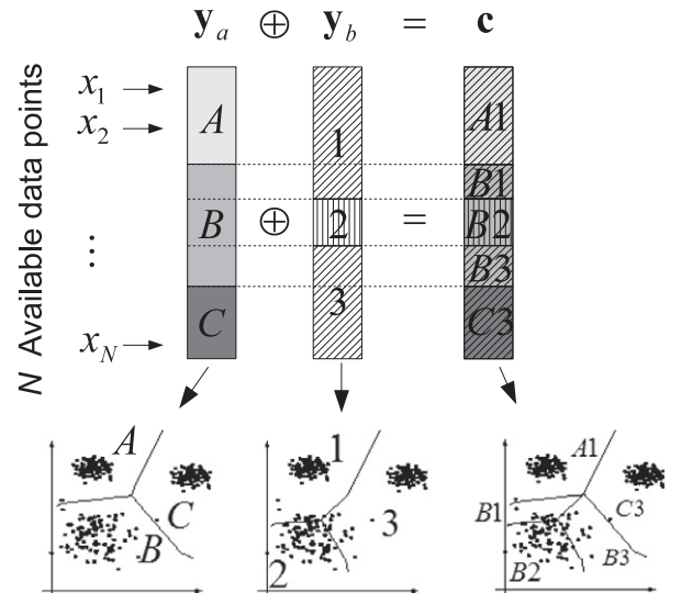
Fig. 2. Concatenation of label vectors as a partition combination.
